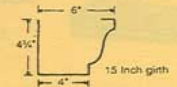
Style K Gutter - dimensions
